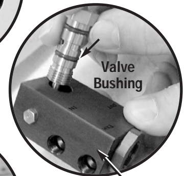
Figure 2 New DVOA
